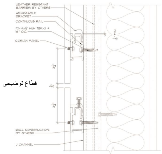
1 400 TYPICAL VERTICAL JOINT SCALE: 1/8" = 1'-0" ARCH REF: N/A
